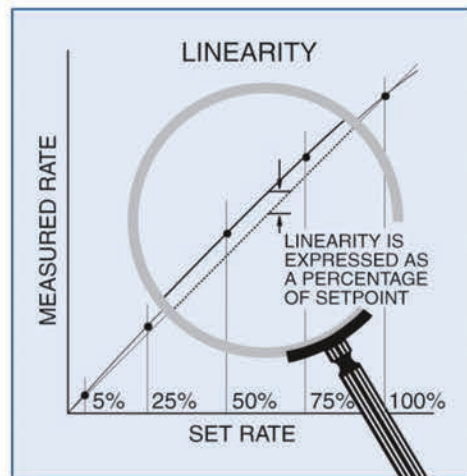
Figure 2. Areas of feeder performance: repeatability, linearity and stability
